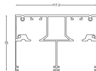
SCP - 62 Sliding Track Size : 6 mtr. Finish : Black Matt
