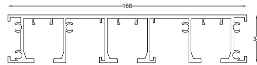
SCP - 58 3 Track Top Size : 6 mtr. Finish : Black Matt
