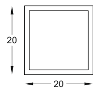
SCP - 07 - 02 Sticking Profile (Hollow) Size : 3 mtr. Finish : Black Matt
