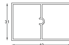
SCP - 133 Door Middle Profile Size : 3 mtr. Finish : Aluminium
