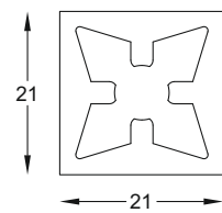
SCP - 07 - 01 Sticking Profile (Vertical) Size : 3 mtr. Finish : Black Matt
