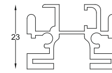
SCP - 111 Wall Panel Profile Size : 2.8 mtr. Finish : Aluminium Matt
