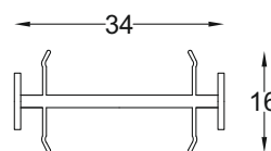
SCP - 60 Sliding Track Jointer Size : 6.3 mtr. Finish : Black Matt
