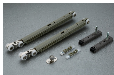
SCPR - 85 2 Door Sliding System (2 Way Soft Close) Finish : Zinc
