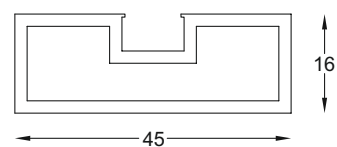
SCP - 51 Frame Profile Size : 4.8 mtr., 6 mtr. Finish : Black Matt
