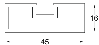
SCP - 51 Frame Profile Size : 4.8 mtr., 6 mtr. Finish : Black Matt
